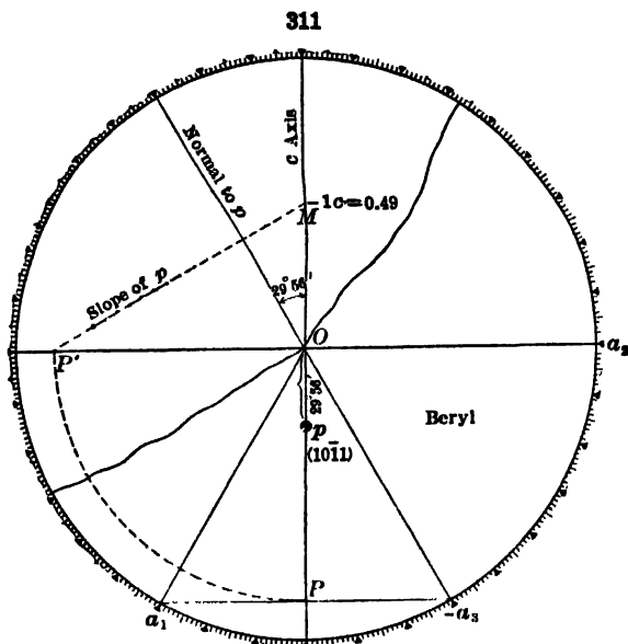
Determination of unit length of c axis, having given the position of p(10\bar{1}1)
